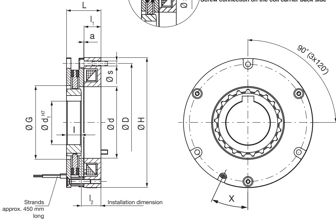
Type 8982.00001 Screw connection on the coil carrier back side
